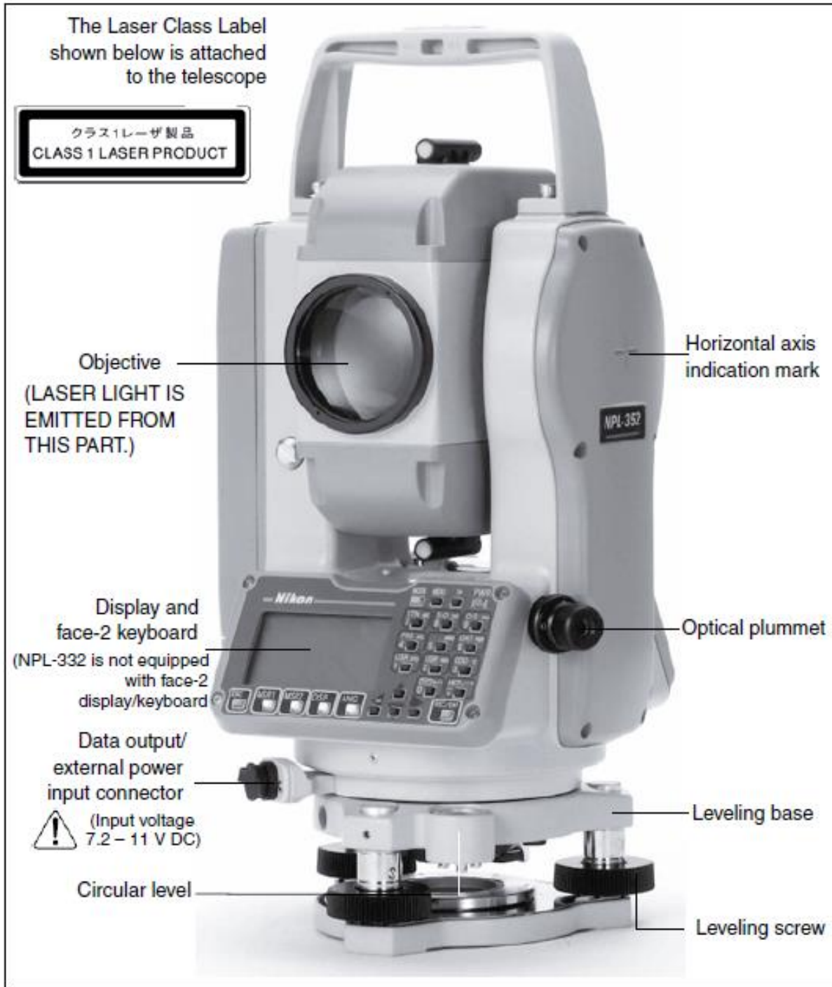
Figure 1.2 Pulse Laser Station NPL-302 series – Face-2
