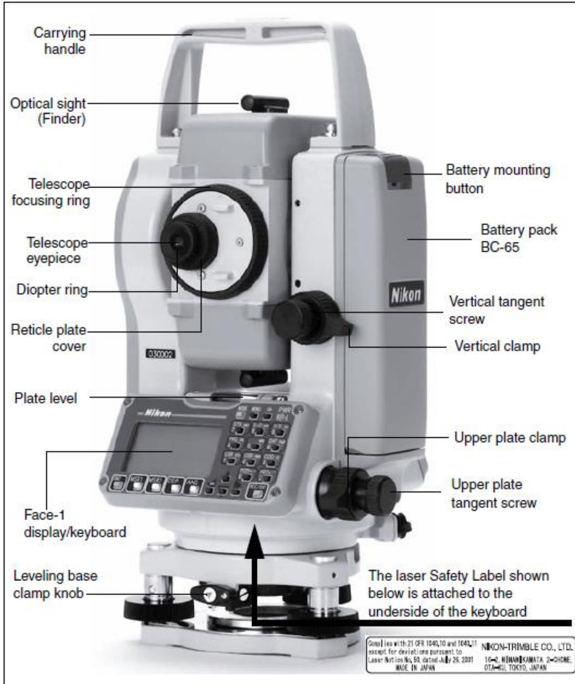
Figure 1.1 Pulse Laser Station NPL-302 series – Face-1
